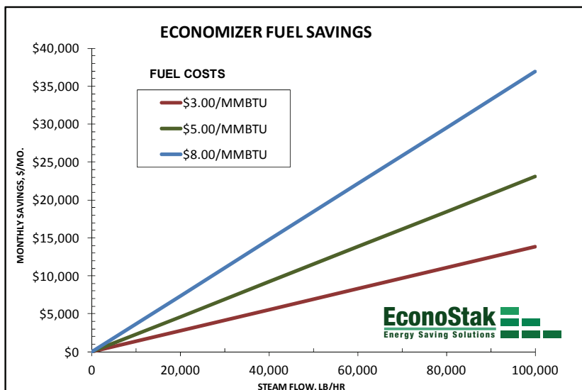
Chart below: Typical performance and monthly savings of an EconoStak economizer at varying steam flows.
